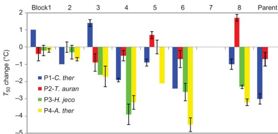
Fig. 3 Changes in the T_{50} values ( ^{\circ}\text{C} ) relative to T. emersonii ( T_{50} = 62.9 \pm 0.3^{\circ}\text{C} ) parent for 28 CBH I monomers. Monomers contain single-block substitutions from parents 1–4 into parent 5 (from T. emersonii ). Error bars for monomers represent the extreme values of two duplicate measurements. Error bars for parents represent the standard deviations for between 3 and 8 replicates. T_{50} values for respective C. thermophilum and T. aurantiacus parent CBH Is are 59.9 \pm 0.3^{\circ}\text{C} and 62.2 \pm 0.4^{\circ}\text{C} . Hypocrea jecorina and A. thermophilum parent CBH Is were not secreted.
