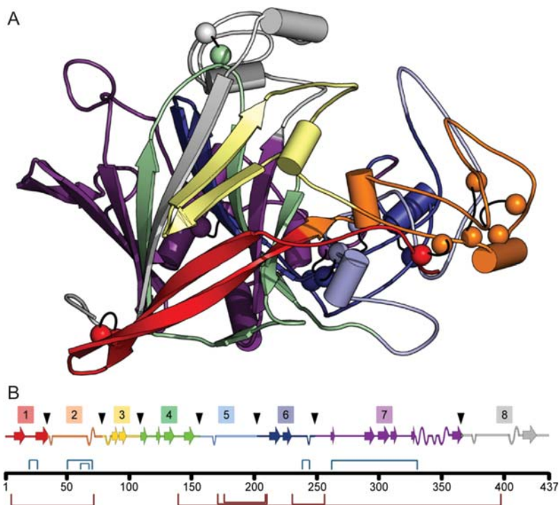
Fig. 1 (A) CBH I catalytic domain three-dimensional structure. Disulfide-bonded Cys residues are denoted by spheres connected by black lines. (B) CBH I recombination block divisions and secondary structure diagram. Interblock disulfide bonds are denoted by maroon lines, intrablock disulfides by light blue lines and block divisions by black arrows. Residue numbering for T. emersonii CBH I.
